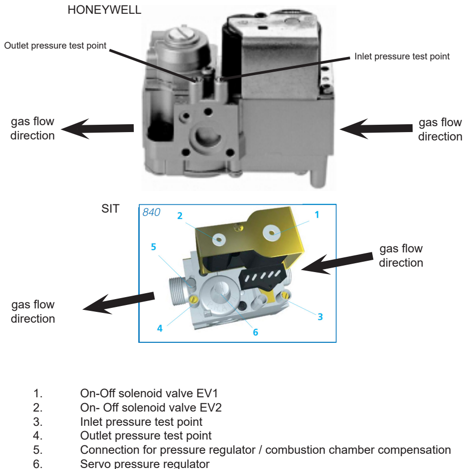
12.picture: Input and output gas pressure checking connections in case of SIT or Honeywell solenoid valve
