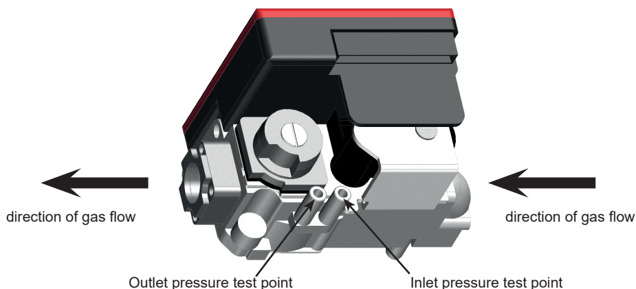
36. picture: Input and output gas pressure checking connections in case of HONEYWELL solenoid valve
