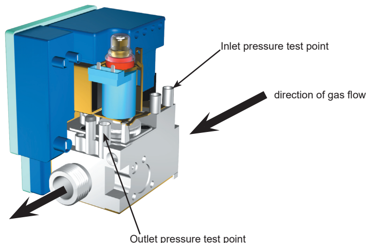
37.picture: Input and output gas pressure checking connections in case of SIT solenoid valve
