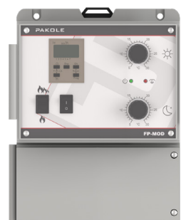
FP-MOD Modulated regulation thermostat with weekly hour programming
