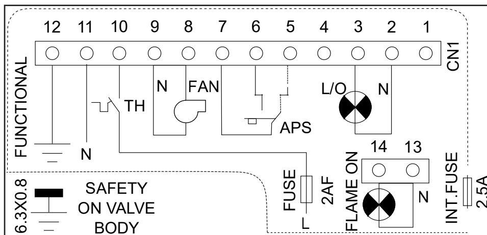
17. picture: Connection points of SIT 579 DBC automatic burner control box
