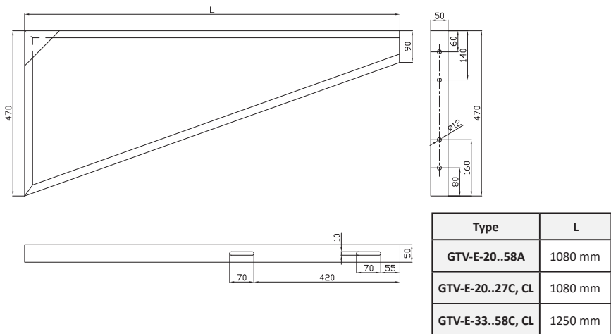
21 picture: Cantilever dimension
