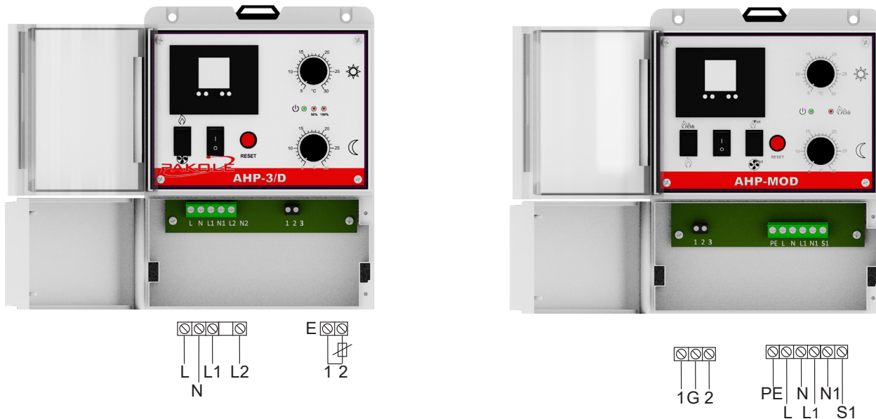
35.picture: AHP-3 and AHP-MOD temperature regulator
